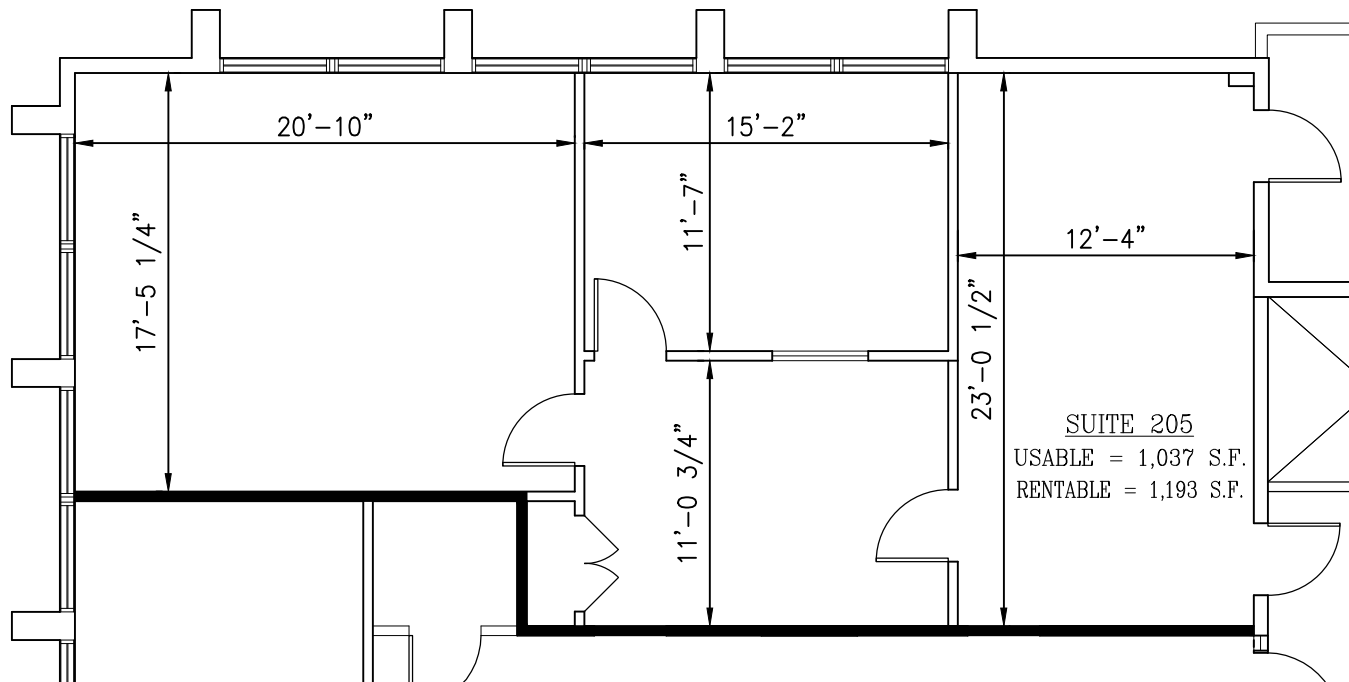
1 SUITE 205 FLOOR PLAN SCALE: 1/8"=1'-0"
