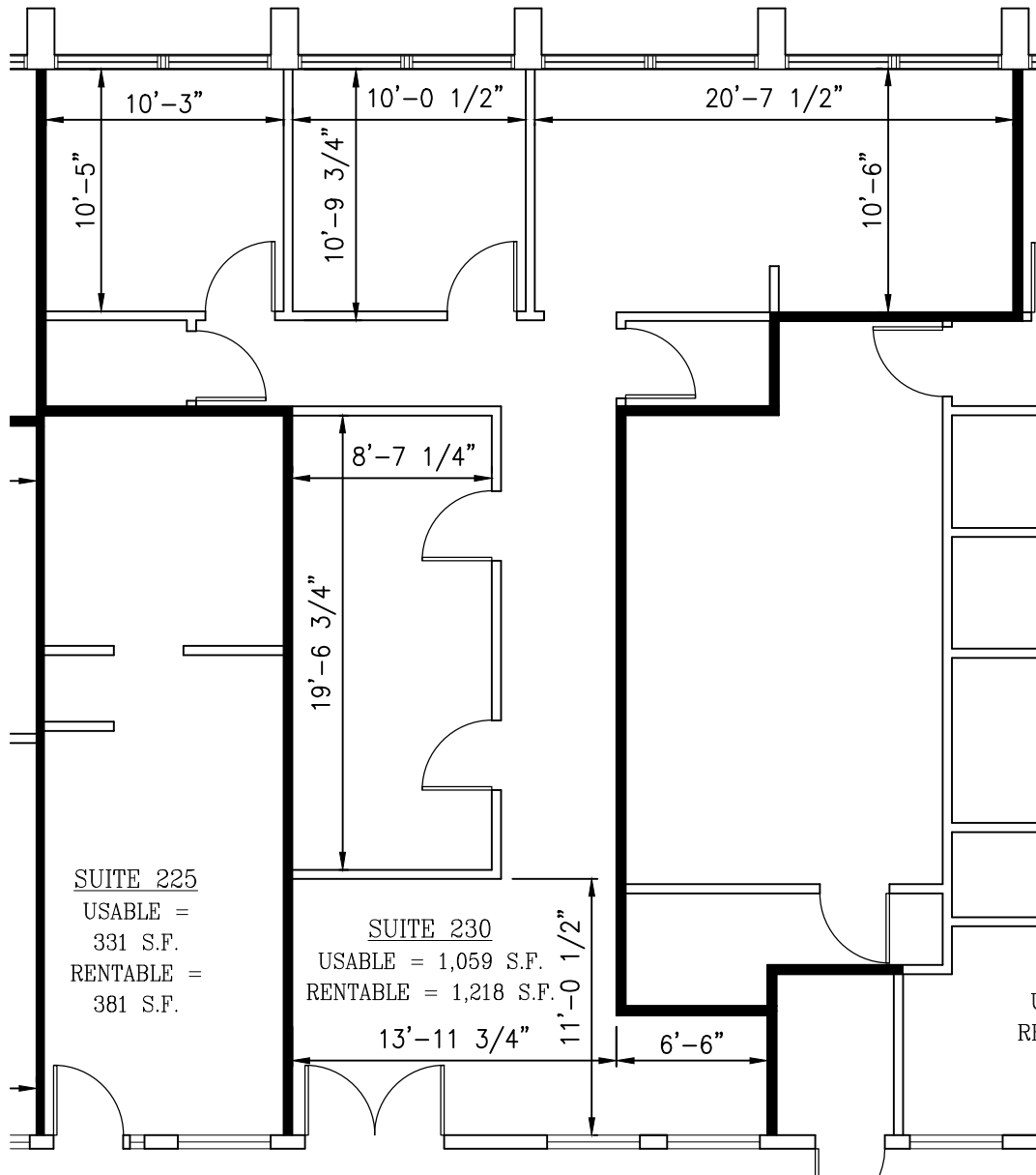
1 SUITE 230 FLOOR PLAN SCALE: 1/8"=1'-0"
