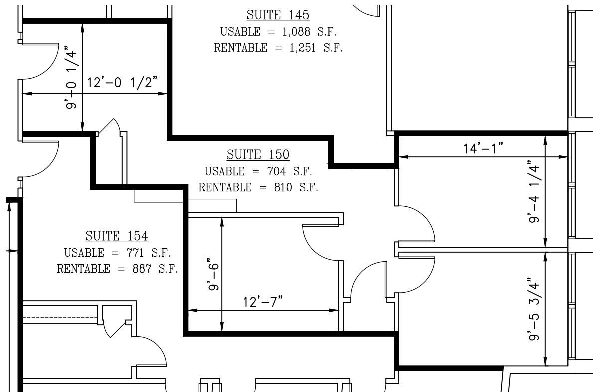
① SUITE 150 FLOOR PLAN SCALE: 1/8"=1'-0"
