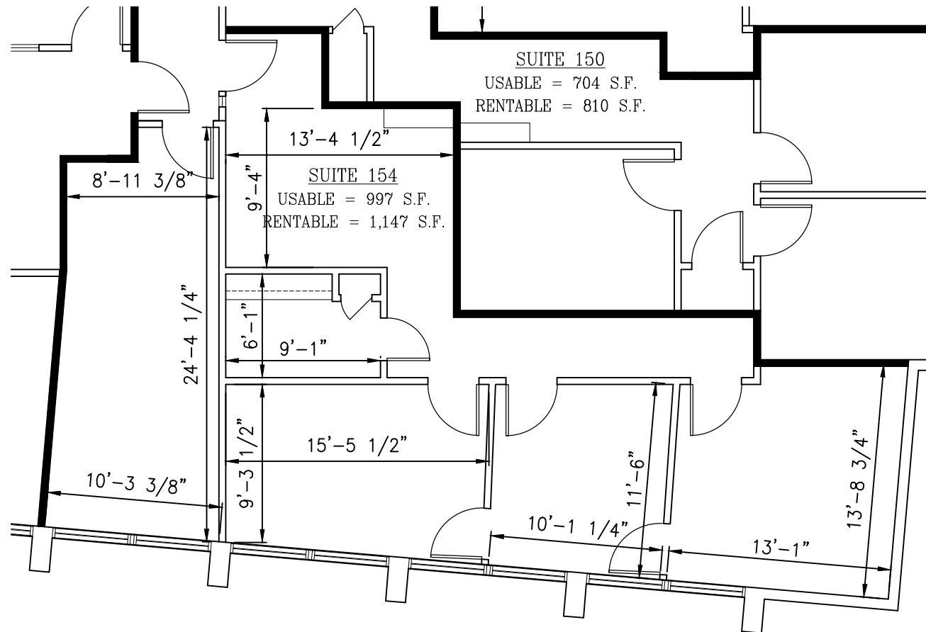
1 SUITE 154 FLOOR PLAN SCALE: 1/8"=1'-0"
