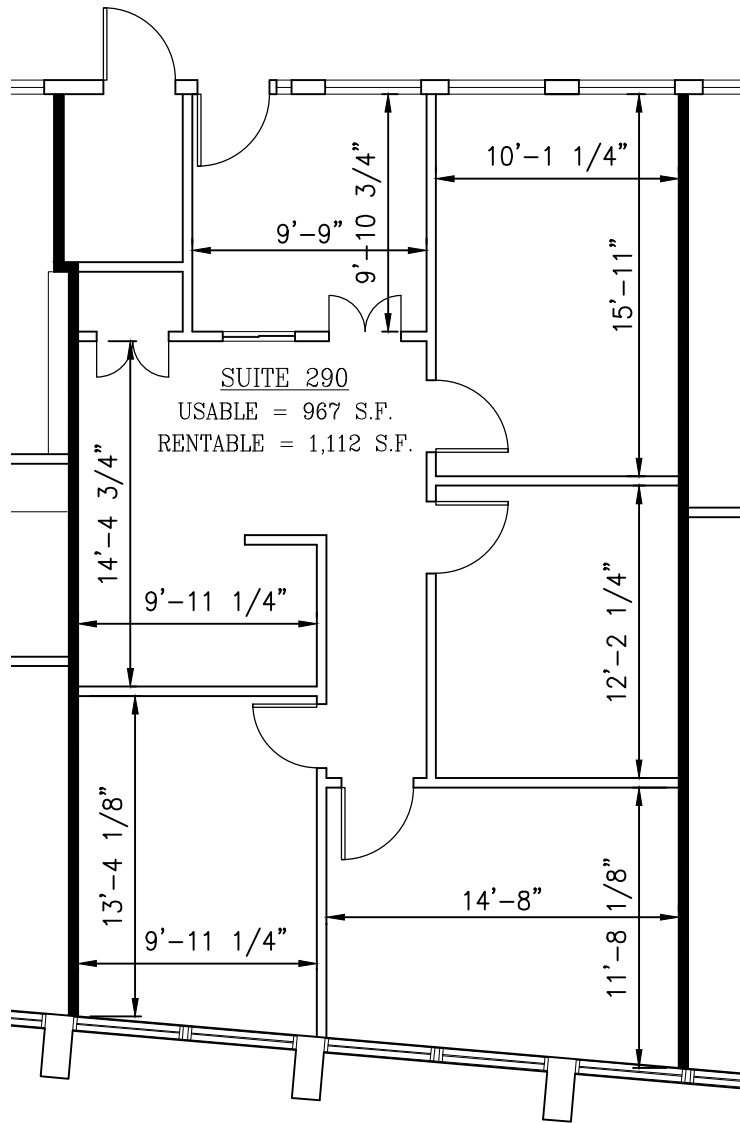
1 SUITE 290 FLOOR PLAN SCALE: 1/8"=1'-0"
