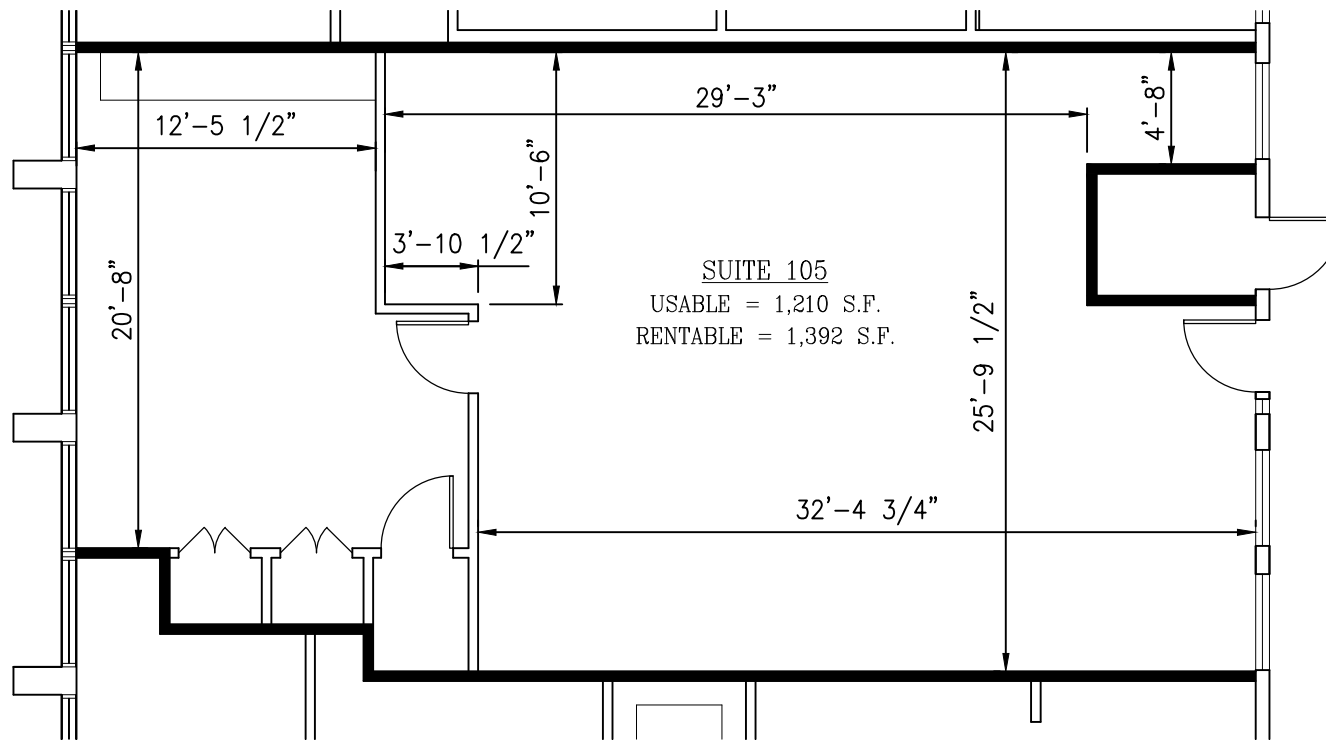
1 SUITE 105 FLOOR PLAN SCALE: 1/8"=1'-0"
