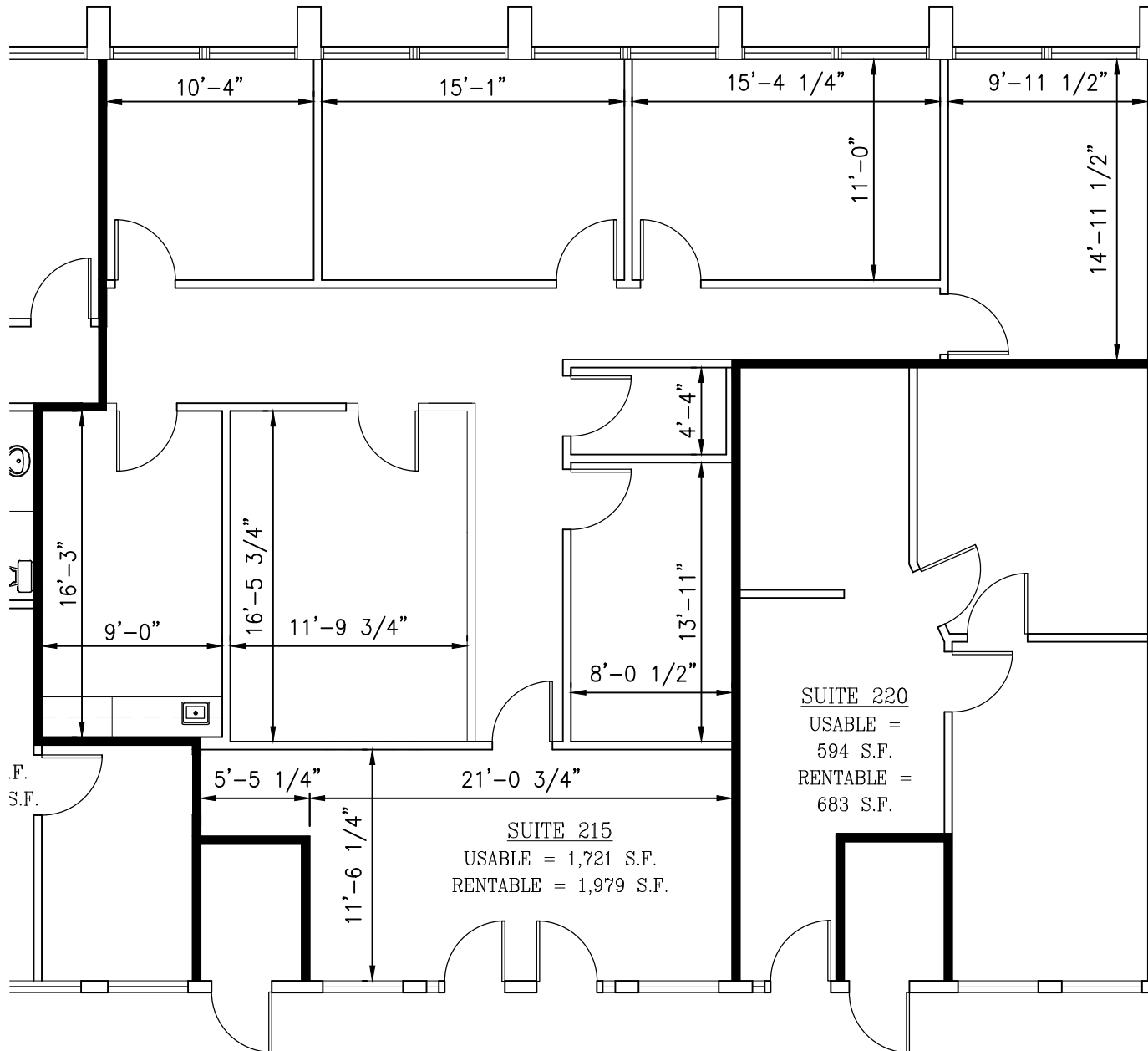
1 SUITE 215 FLOOR PLAN SCALE: 1/8"=1'-0"
