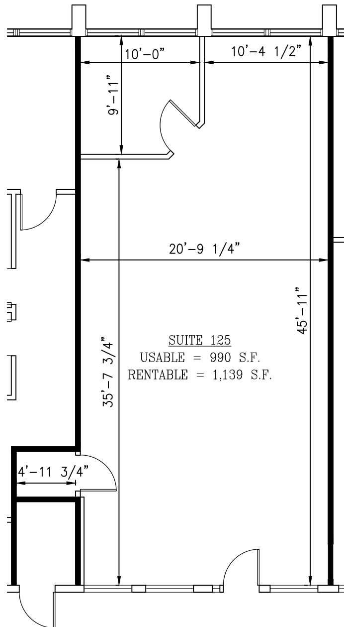
1 SUITE 125 FLOOR PLAN SCALE: 1/8"=1'-0"
