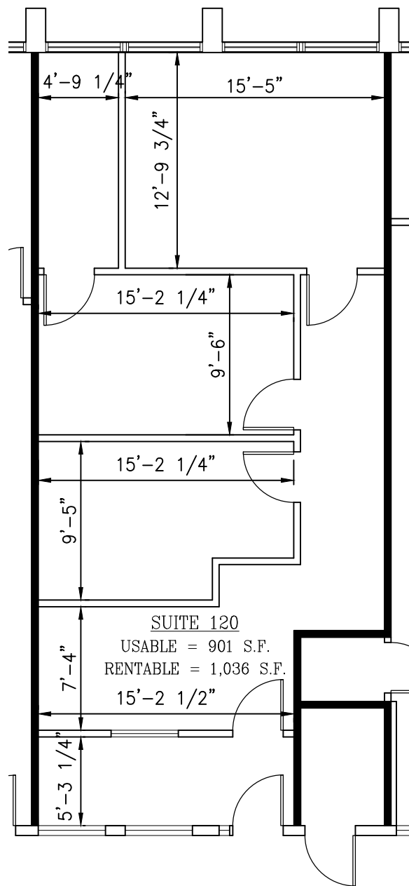
1 SUITE 120 FLOOR PLAN SCALE: 1/8"=1'-0"
