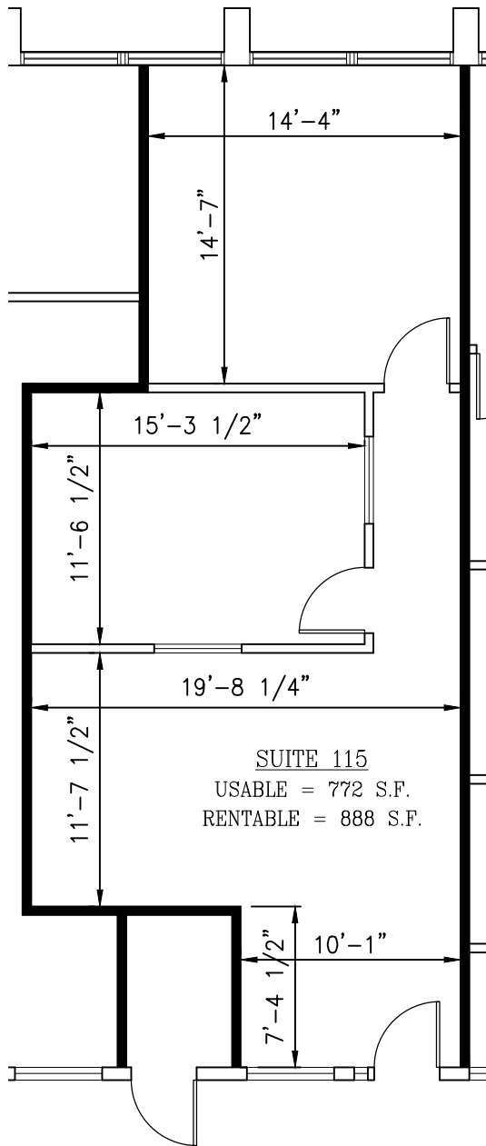
1 SUITE 115 FLOOR PLAN SCALE: 1/8"=1'-0"
