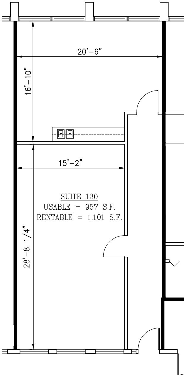
1 SUITE 130 FLOOR PLAN SCALE: 1/8"=1'-0"
