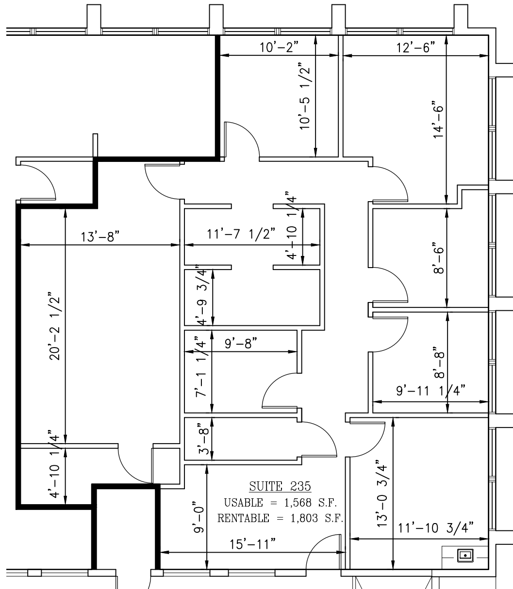
1 SUITE 235 FLOOR PLAN SCALE: 1/8"=1'-0"
