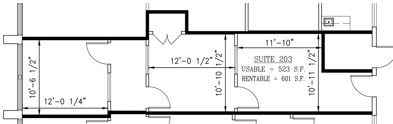
1 SUITE 203 FLOOR PLAN SCALE: 1/8"=1'-0"
