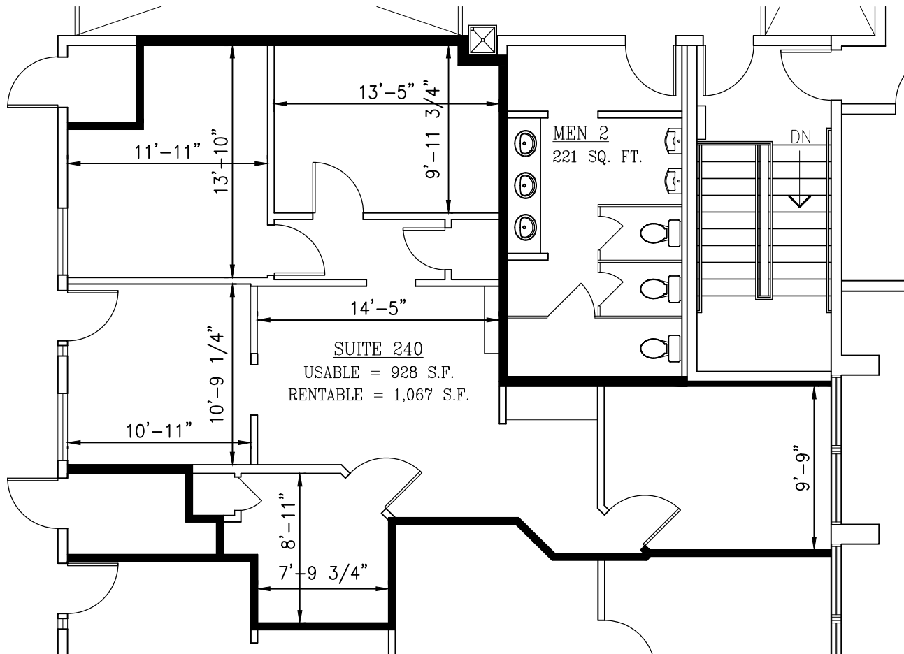
1 SUITE 240 FLOOR PLAN SCALE: 1/8"=1'-0"
