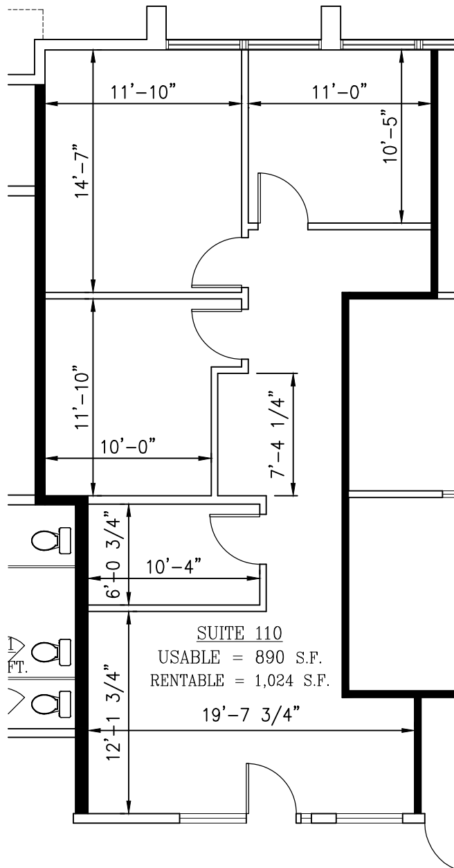
1 SUITE 110 FLOOR PLAN SCALE: 1/8"=1'-0"
