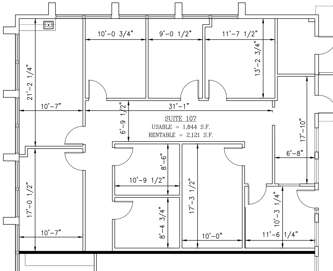
1 SUITE 107 FLOOR PLAN SCALE: 1/8"=1'-0"
