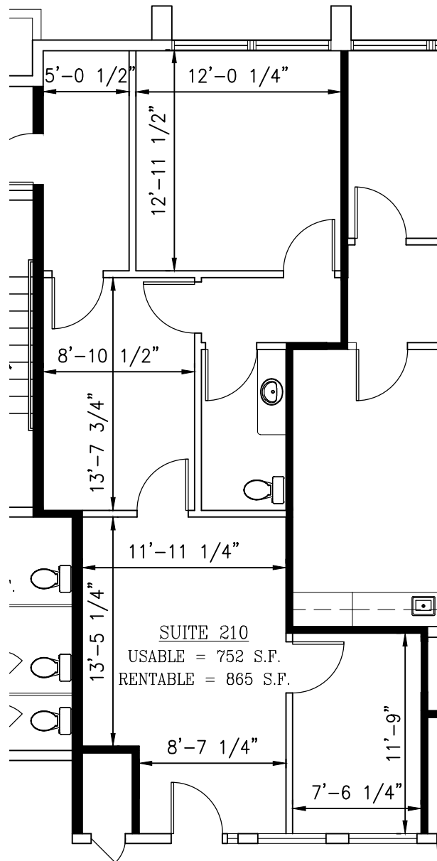
1 SUITE 210 FLOOR PLAN SCALE: 1/8"=1'-0"
