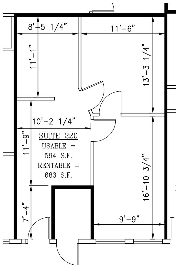
1 SUITE 220 FLOOR PLAN SCALE: 1/8"=1'-0"
