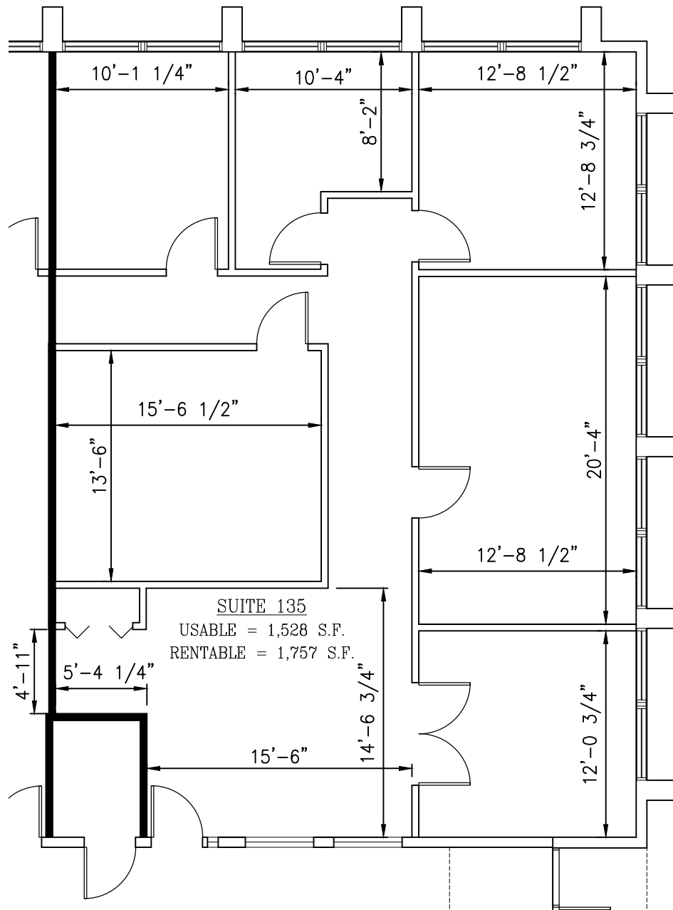
1 SUITE 135 FLOOR PLAN SCALE: 1/8"=1'-0"
