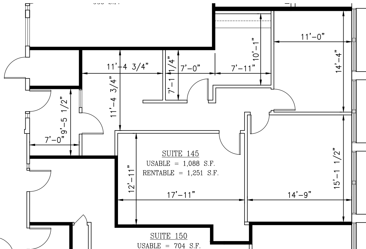
1 SUITE 145 FLOOR PLAN SCALE: 1/8"=1'-0"
