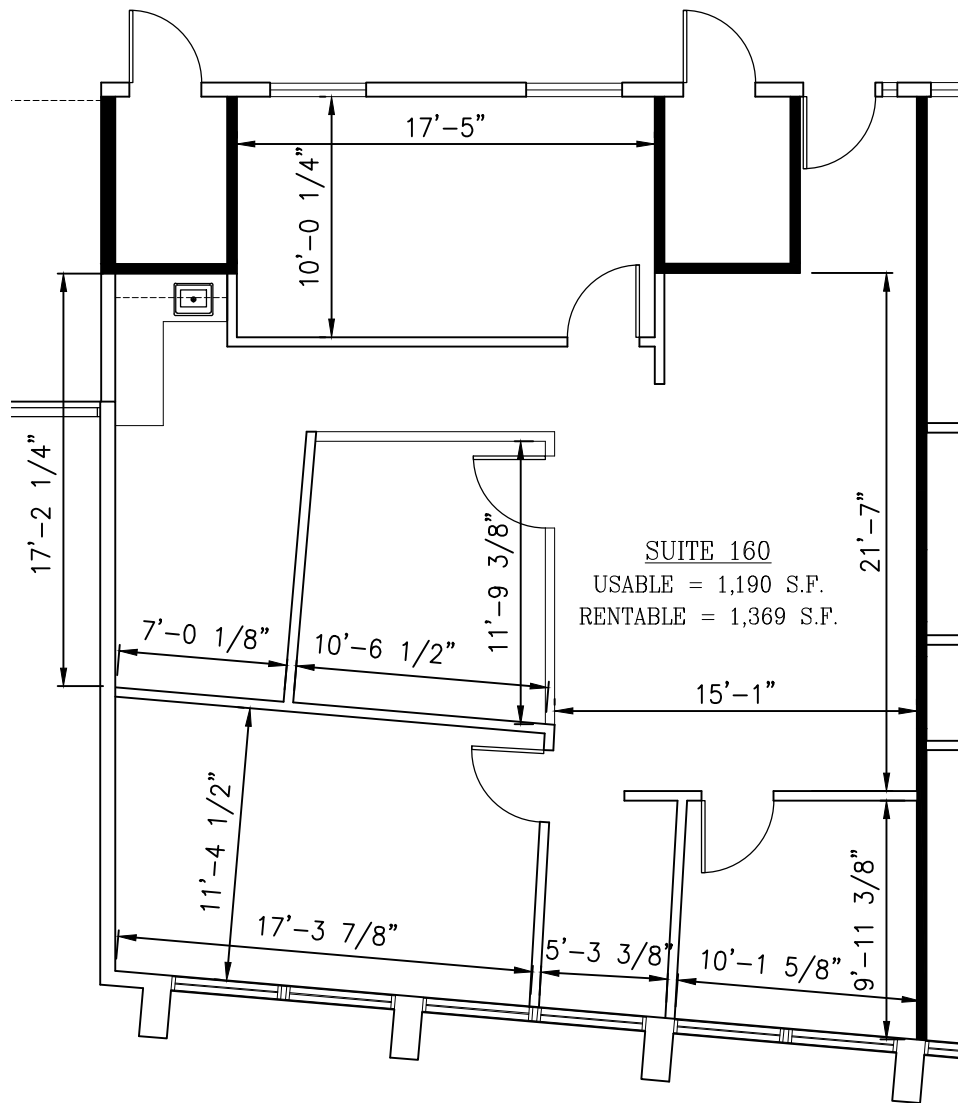
1 SUITE 160 FLOOR PLAN SCALE: 1/8"=1'-0"
