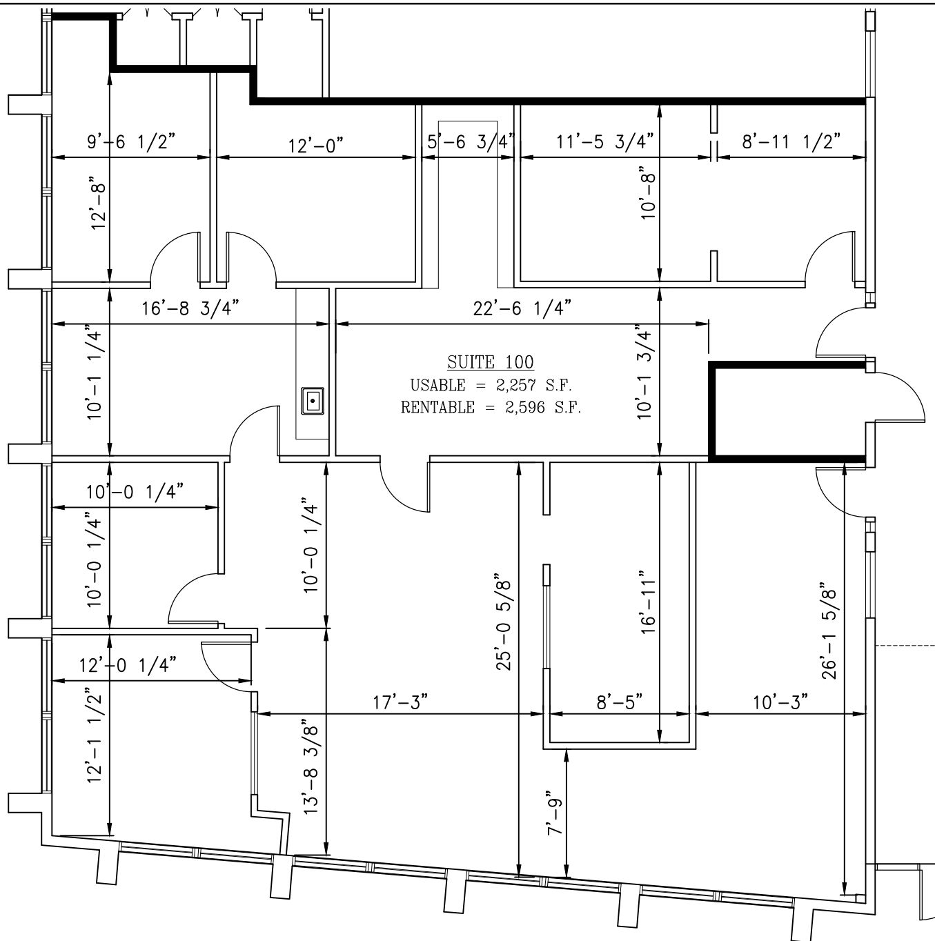
1 SUITE 100 FLOOR PLAN SCALE: 1/8"=1'-0"
